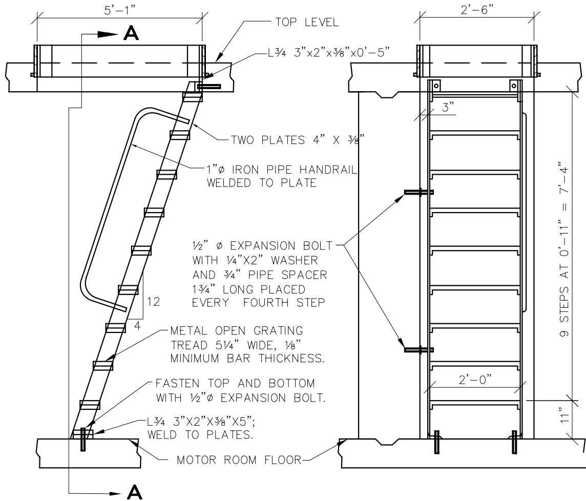
PROFILE
