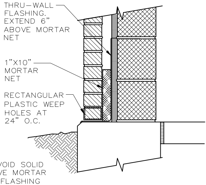
TYP. BASE FLASHING
