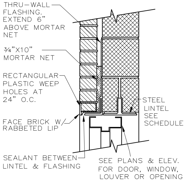
TYP. LINTEL FLASHING
