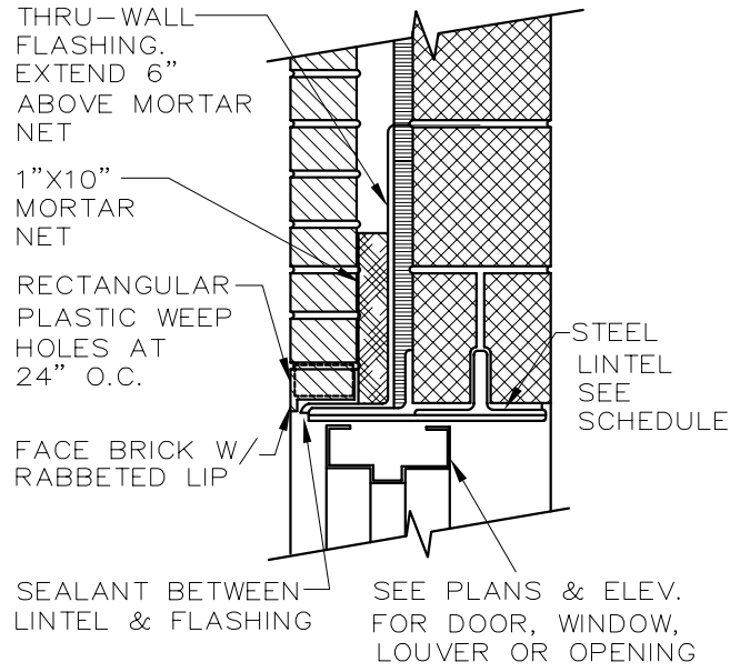
TYP. LINTEL FLASHING
