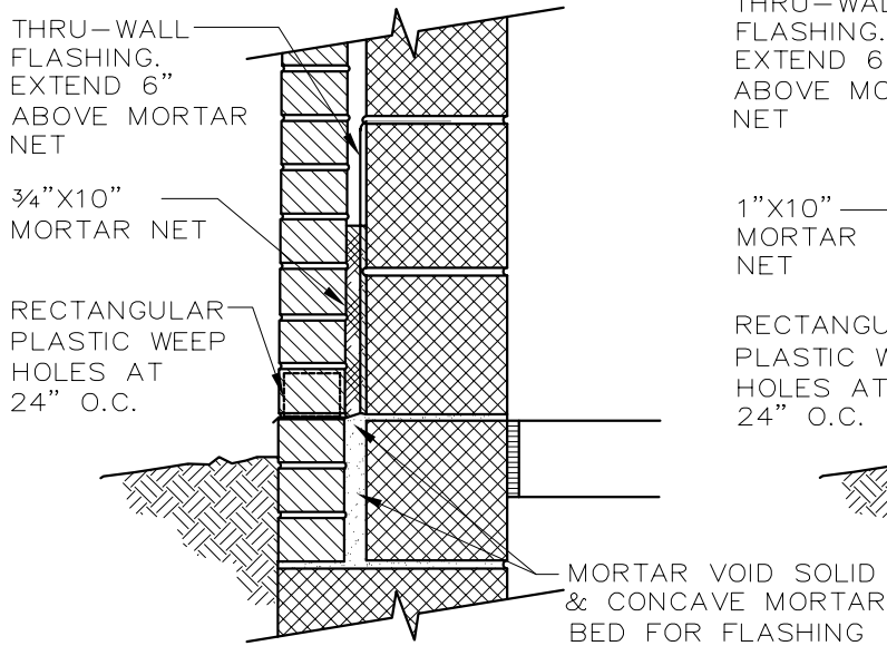
TYP. BASE FLASHING
